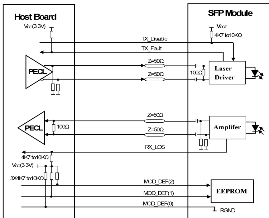
SFP Host Recommended Circuit
