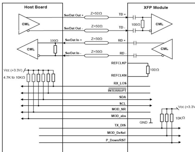
SFP Host Recommended Circuit
