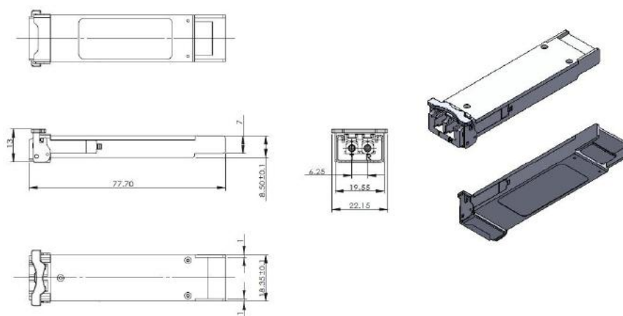
Mechanical Drawing
