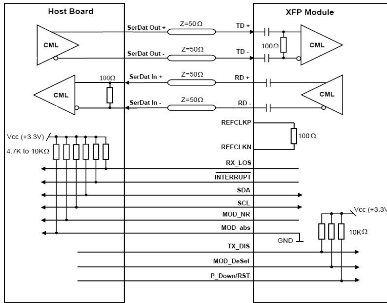
Recommended High-speed Interface Circuit
