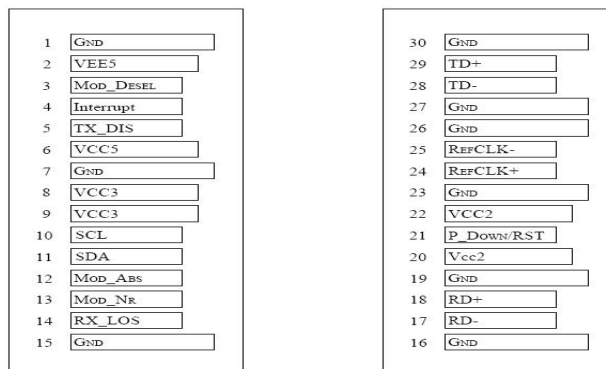
Bottom of Board (As view through top of board)
