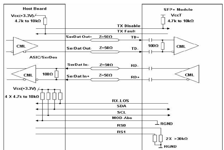
Recommended High-speed Interface Circuit
