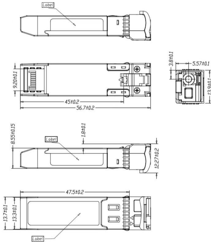
Mechanical Drawing
