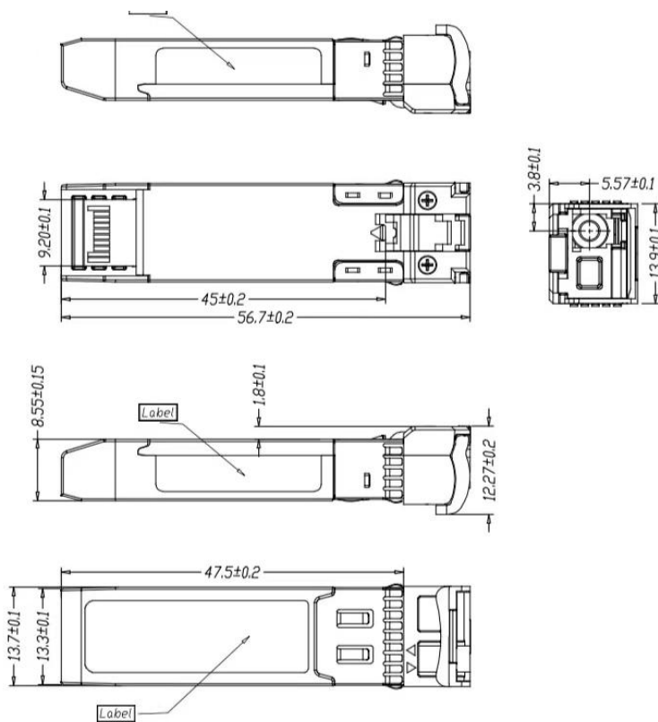
Mechanical Drawing
