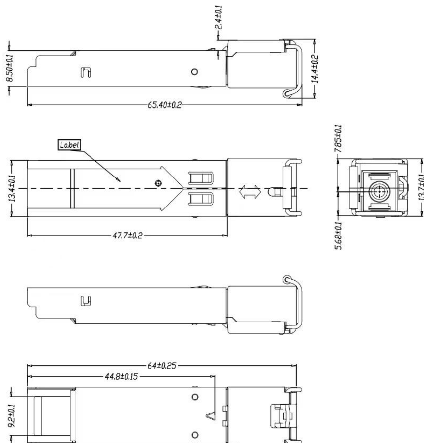
Mechanical Drawing
