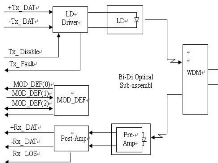
Block Diagram
