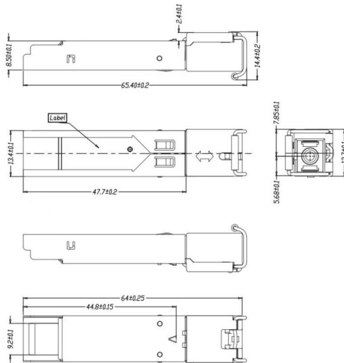
Mechanical Drawing
