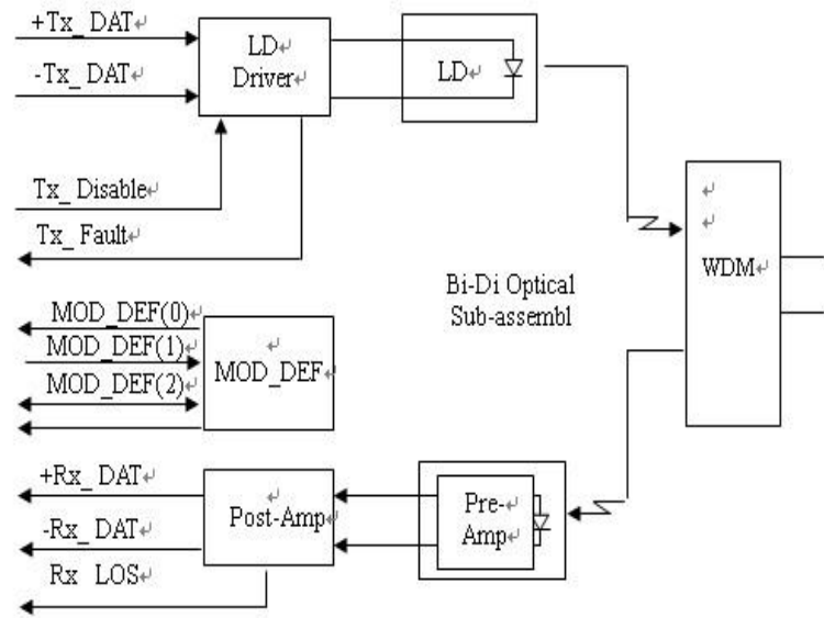
Block Diagram
