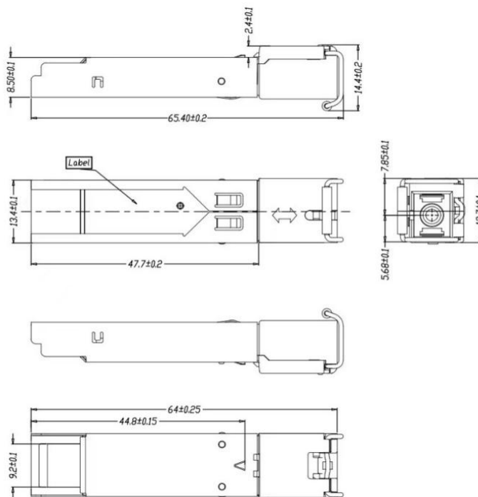
Mechanical Drawing
