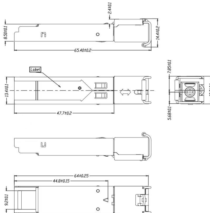
Mechanical Drawing
