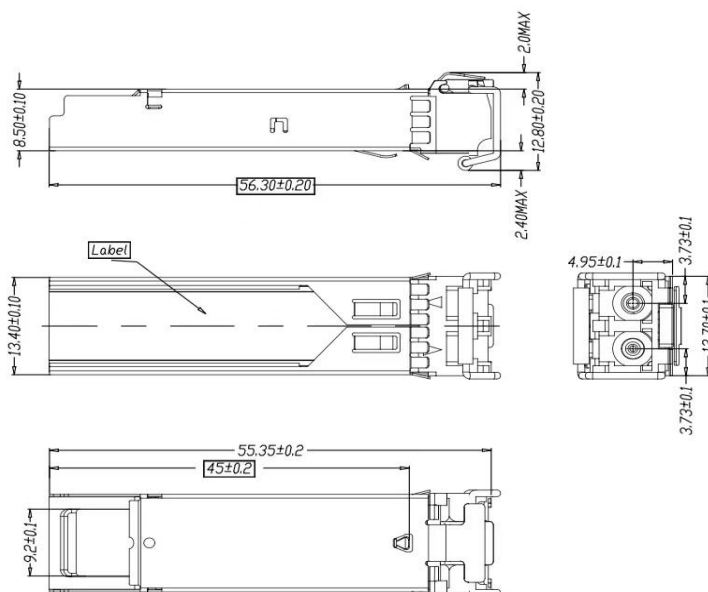
Mechanical Drawing
