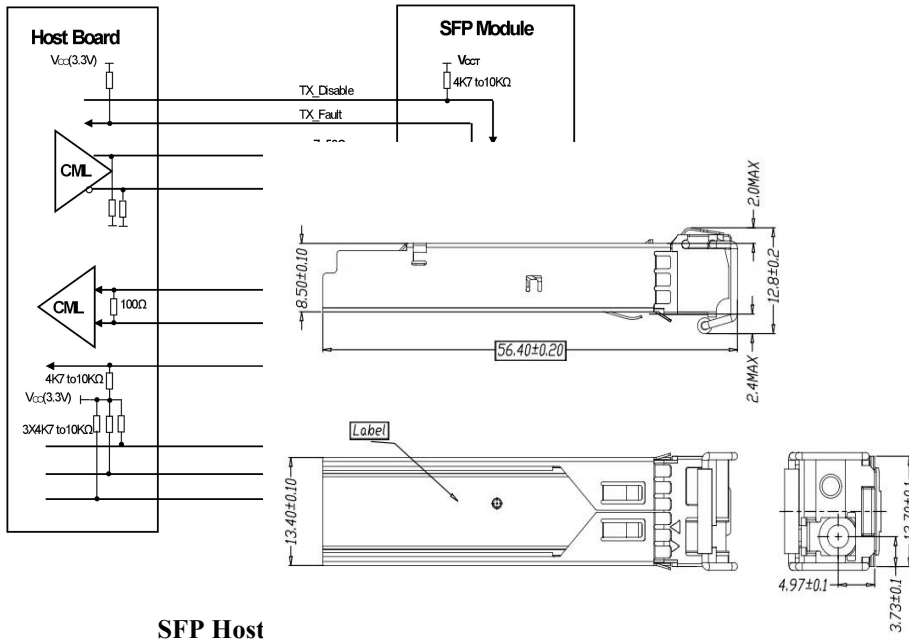
SFP Host
