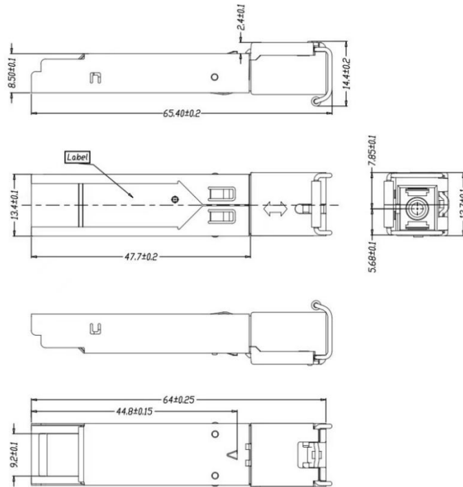
Mechanical Drawing
