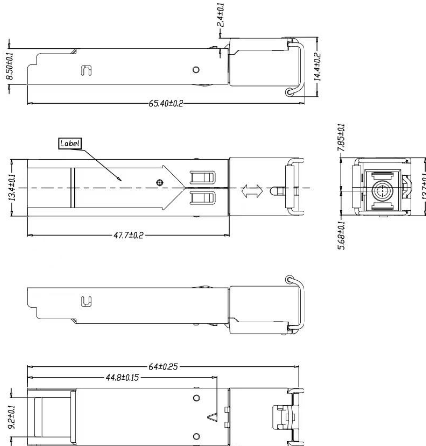
Mechanical Drawing
