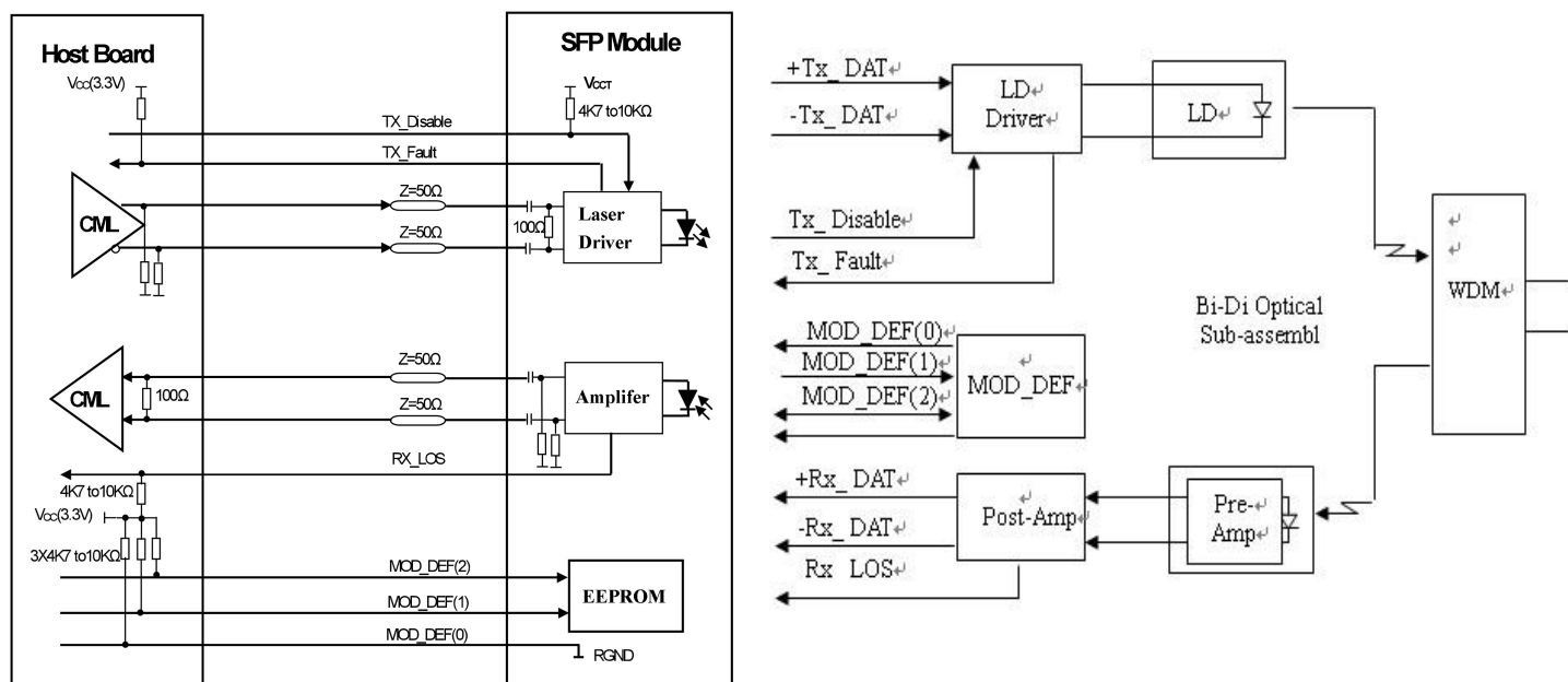
SFP Host Recommended Circuit Block Diagram
