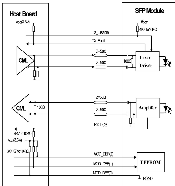
SFP Host Recommended Circuit
