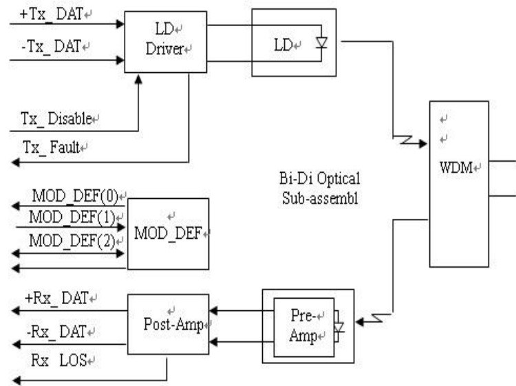
Block Diagram
