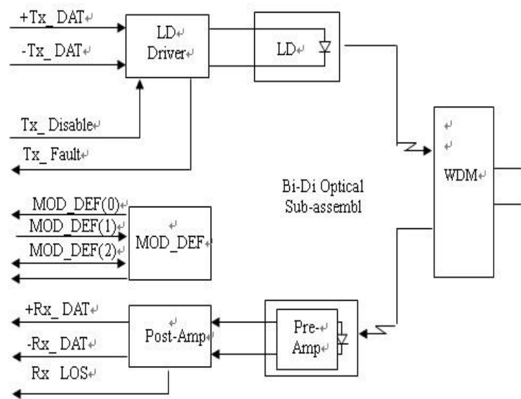
Block Diagram
