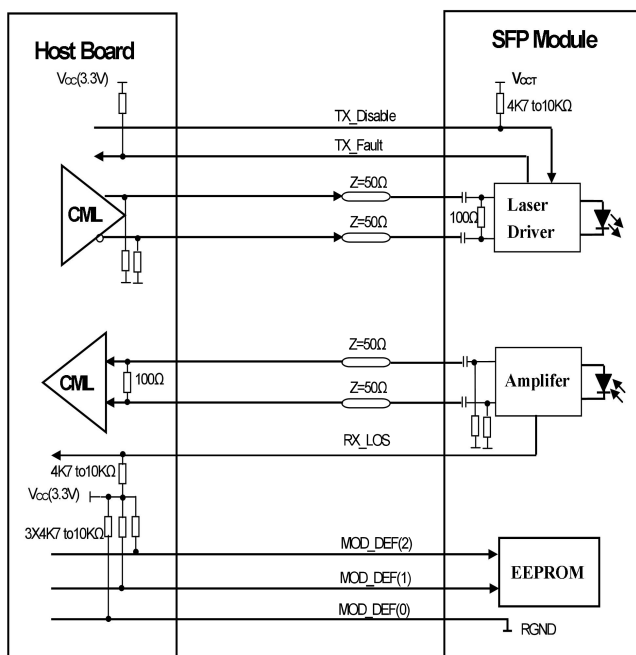
SFP Host Recommended Circuit
