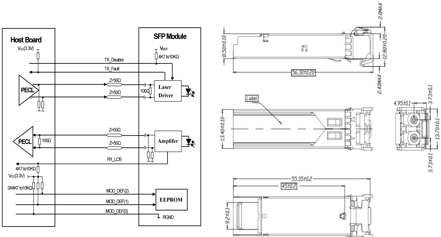
SFP Host Recommended Circuit
