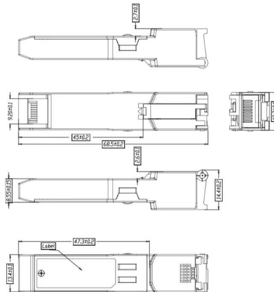
Figure 2. Mechanical Dimensions of Transceiver
