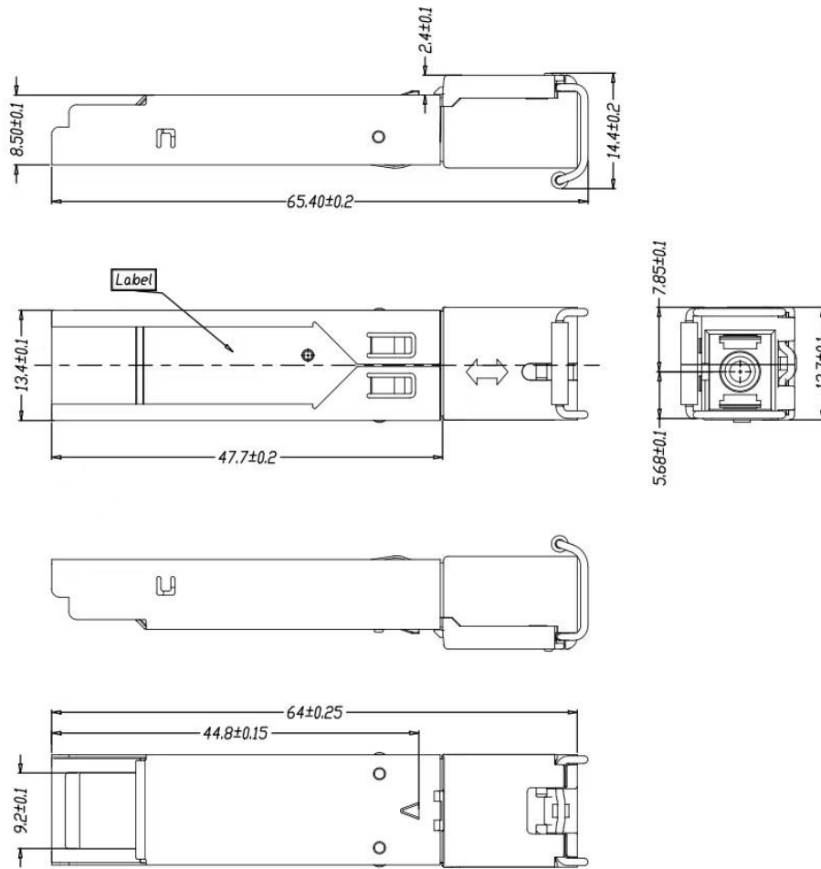
Mechanical Drawing
