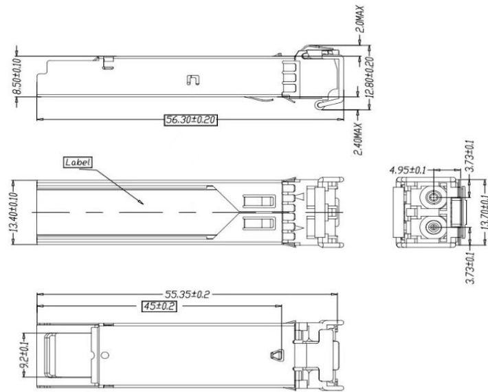
Mechanical Drawing
