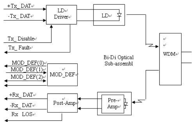
Block Diagram
