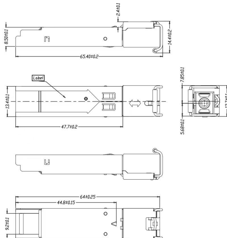
Mechanical Drawing
