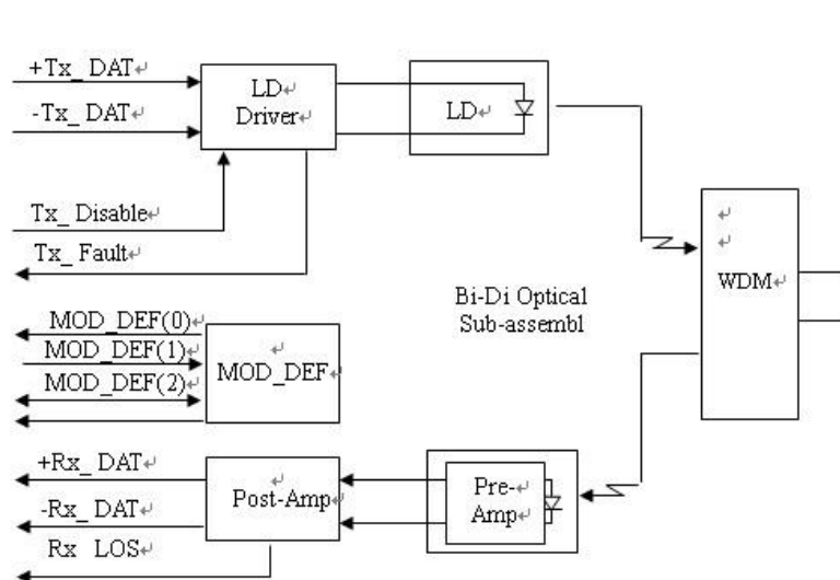
Block Diagram
