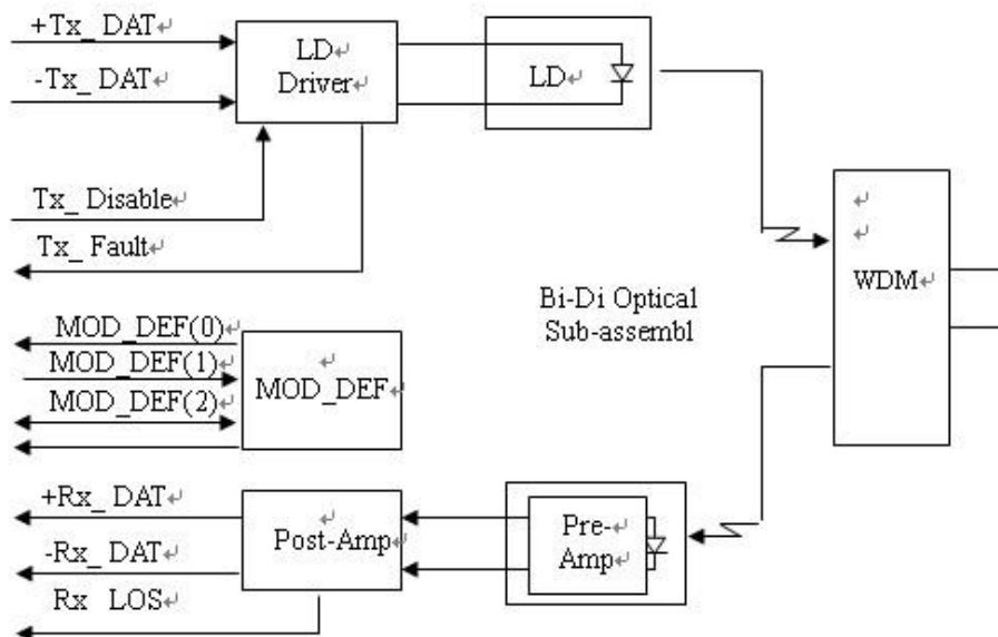
Block Diagram
