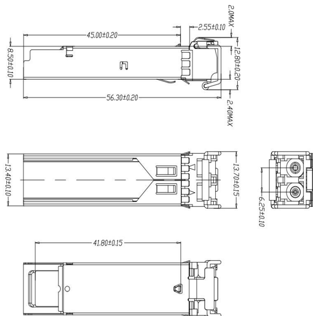
Mechanical Drawing
