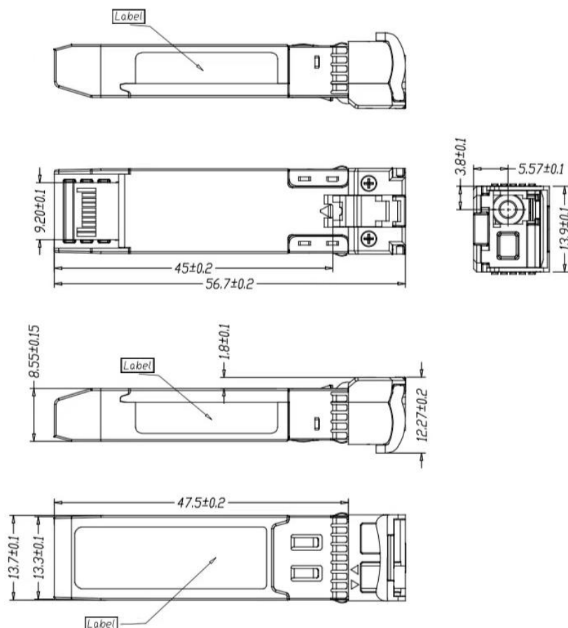
Mechanical Drawing
