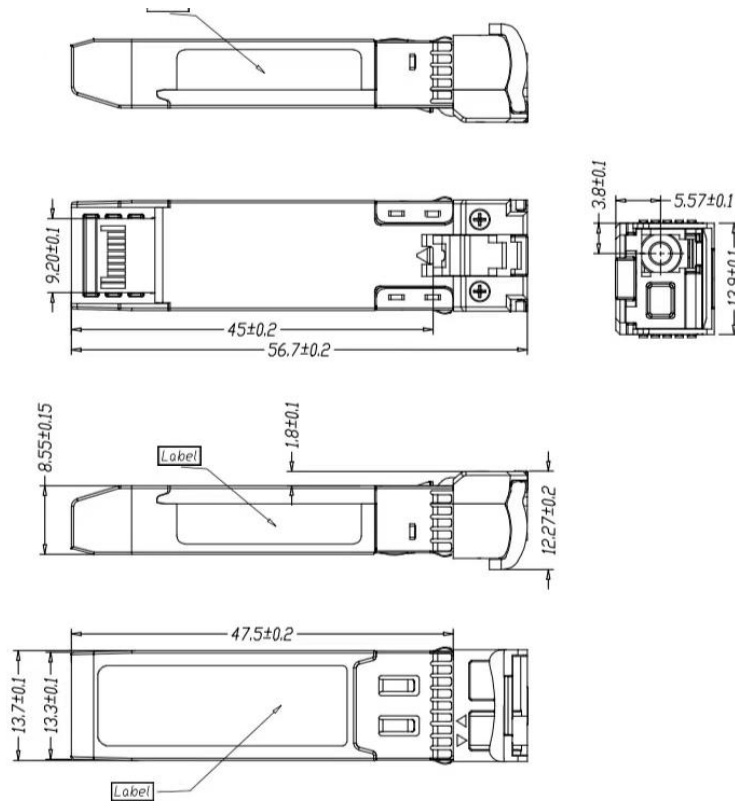
Mechanical Drawing
