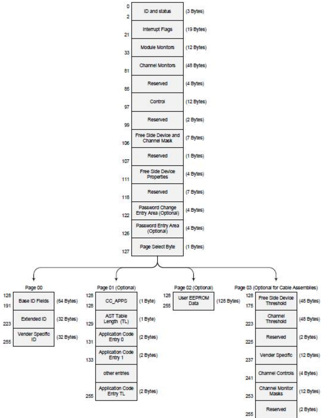
QSF Memory Map
