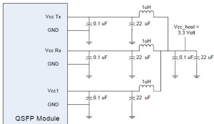
Recommended Host Board Power Supply Filtering
