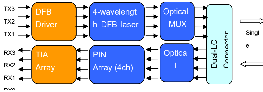
Figure 1: 40Gb/s QSFP IR4 Transceiver Block
