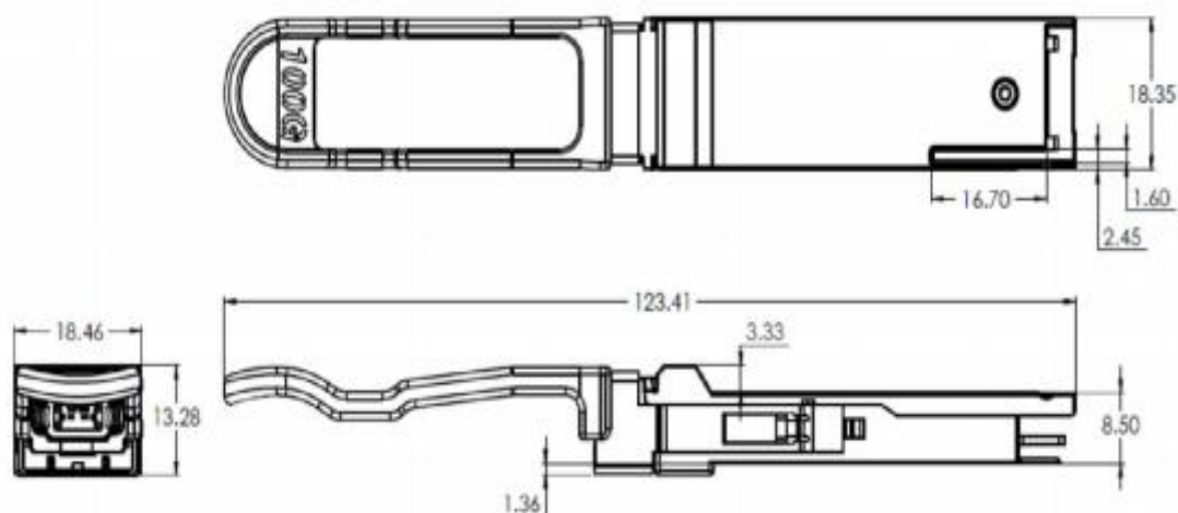
Mechanical Dimensions
