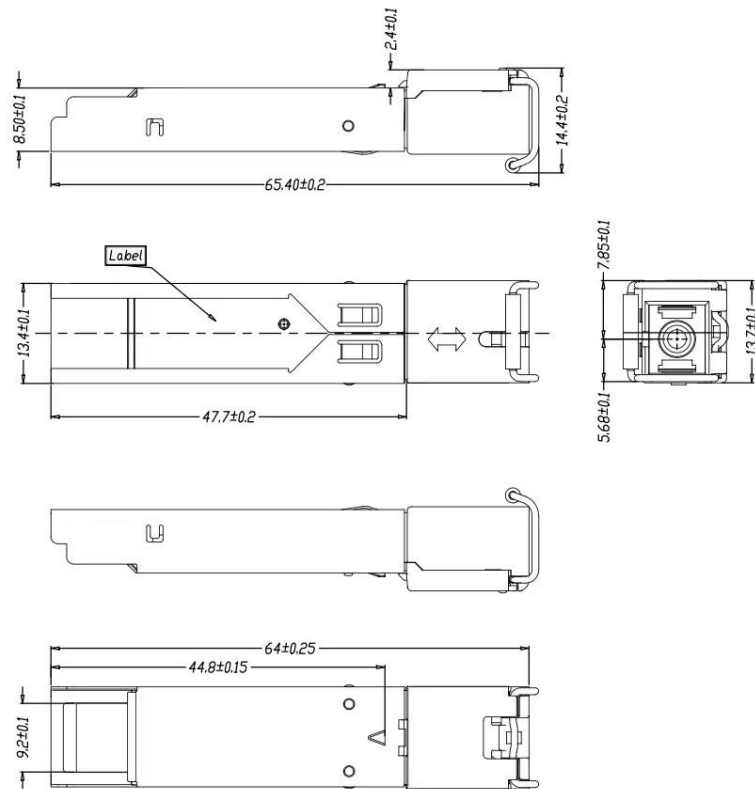
Mechanical Drawing
