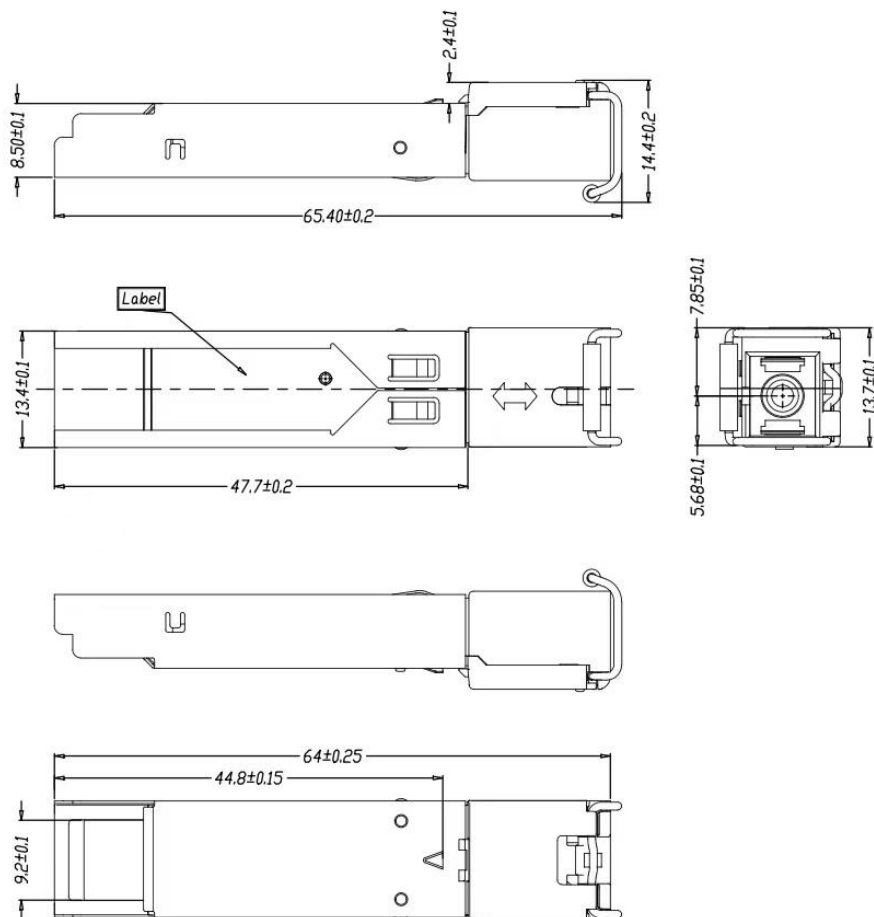
Mechanical Drawing
