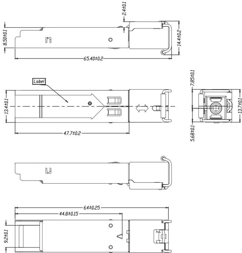
Mechanical Drawing
