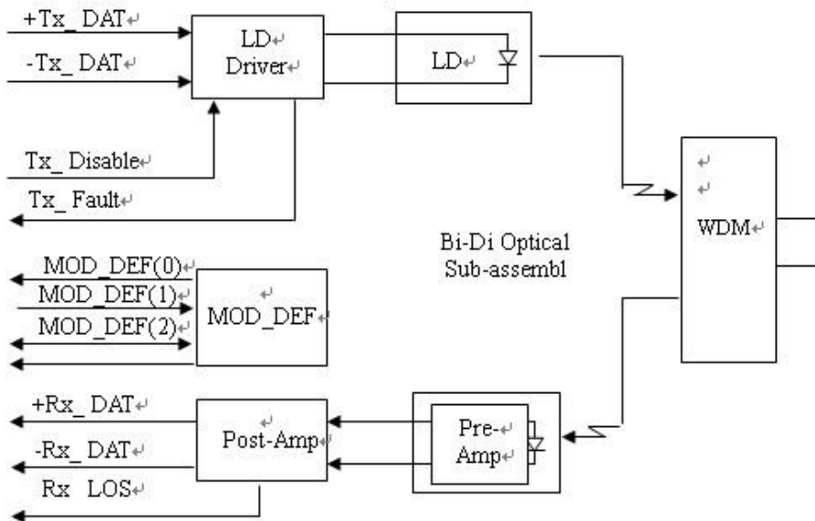
Block Diagram
