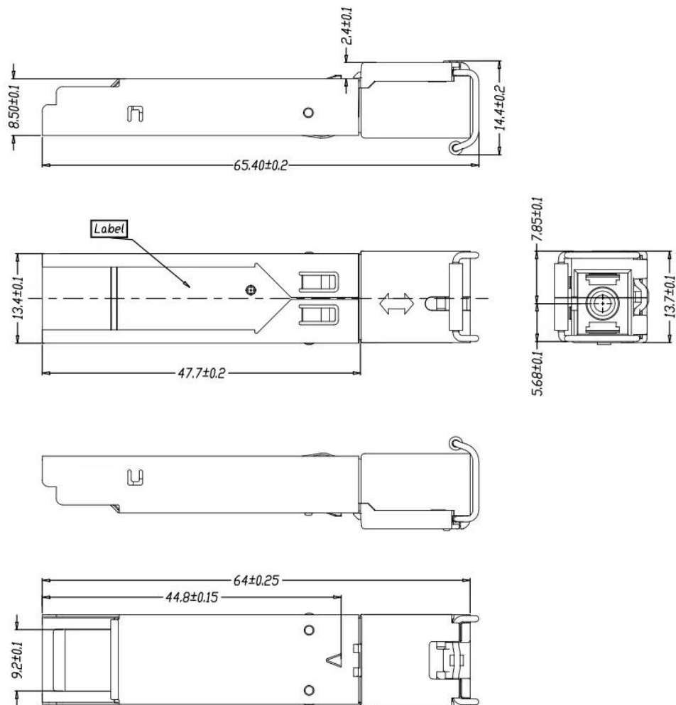
Mechanical Drawing
