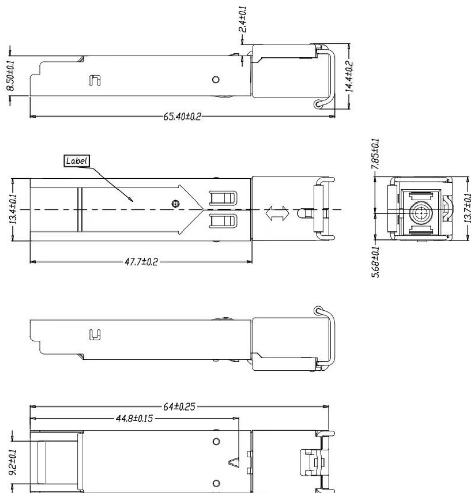
Mechanical Drawing
