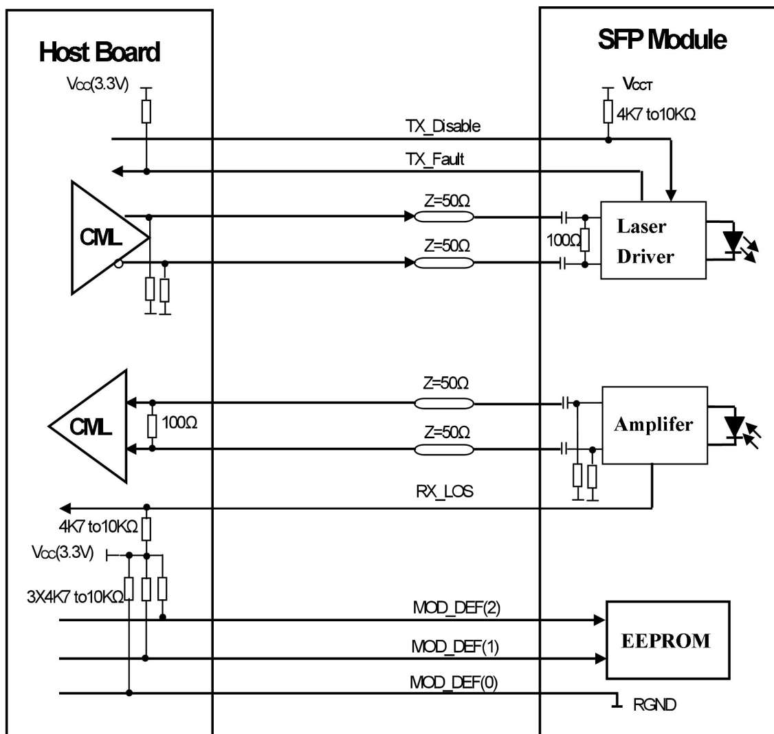
SFP Host Recommended Circuit
